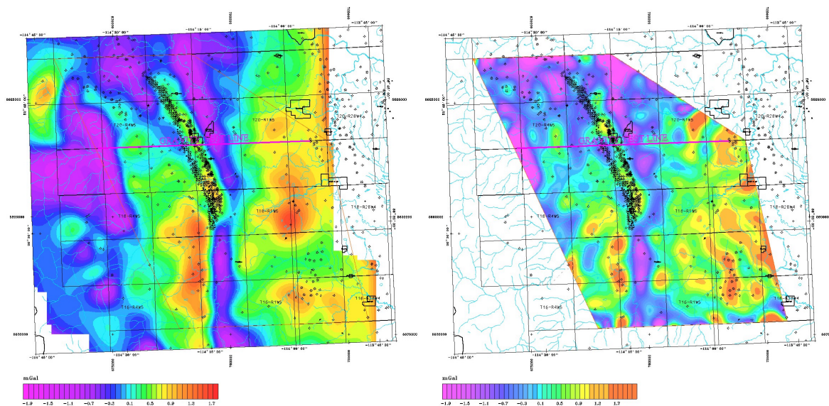
Figure 3 - First Vertical Derivative (1VD) of complete Bouguer Gravity. The left image is the 1VD of the ground gravity data in Fig. 2. The right image is the 1VD of the airborne gravity in Fig. 2. Most of the differences in these maps reflect the additional detail derived from the uniform sampling of the airborne gravity survey.
