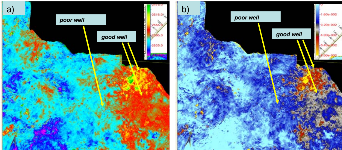
Figure 4. Horizon slice at Cadomin+6ms of the (a) density results from neural network analysis and (b) porosity results from the inverted density response using a standard linear-density relationship. Note the distinct separation of sand from silt and shale.
