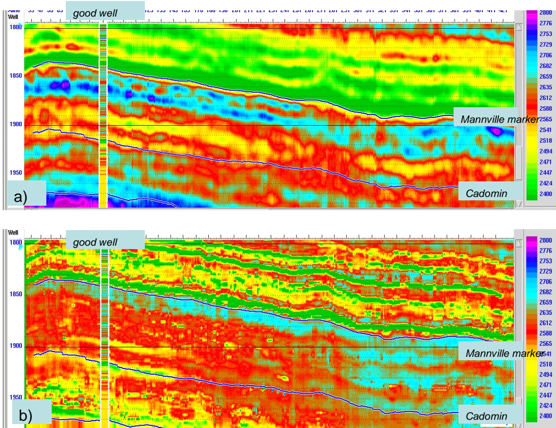
Figure 3: Density results from (a) simultaneous inversion and (b) neural network analysis. Inserted in color is the density log which correlates much better with neural network results
