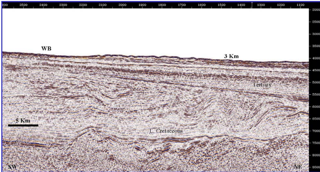
Figure 1. Compressional structures from the Labrador Sea rifted area (data courtesy of GSI).
