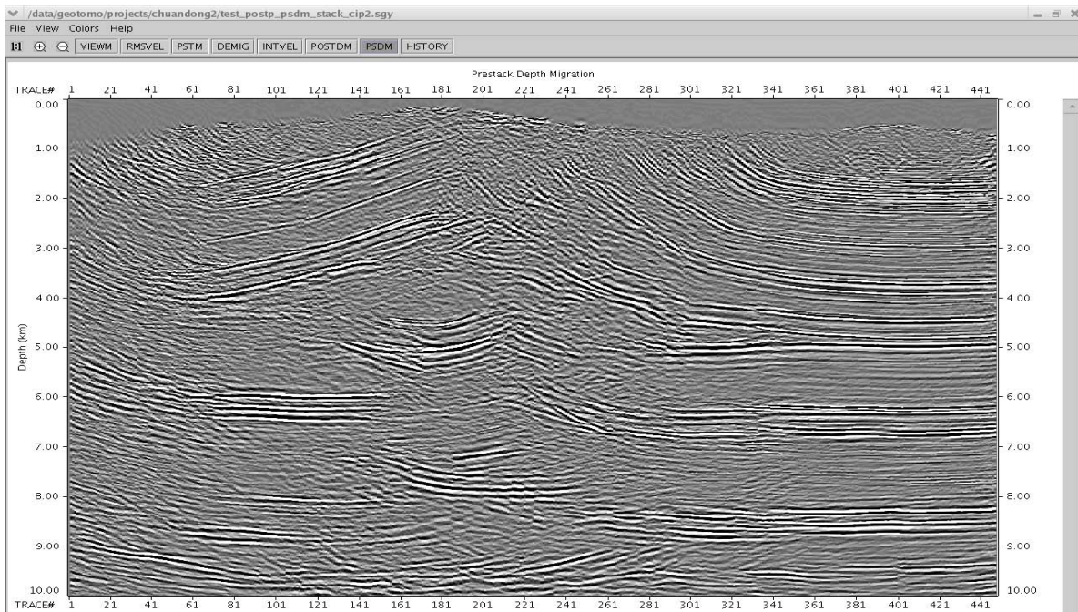
Figure 3. Image from prestack depth migration using velocity-depth model based on layer-by-layer half-space velocity analysis.
