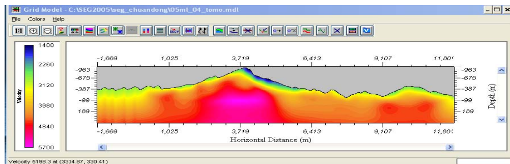
Figure 1. The near-surface model estimated by nonlinear inversion of the traveltimes associated with the first arrivals on shot
