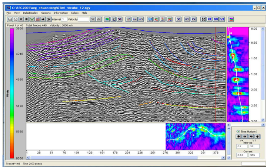
Figure 2. The X-T (top), V-T (right), and V-X (bottom) cross-sections of the rms velocity-cube. The image panels in the X-T lane are used to pick horizon strands and the semblance spectra in the V-X plane are used to pick velocity strands, while the semblance spectrum in the V-T plane is used to quality control the picks.
