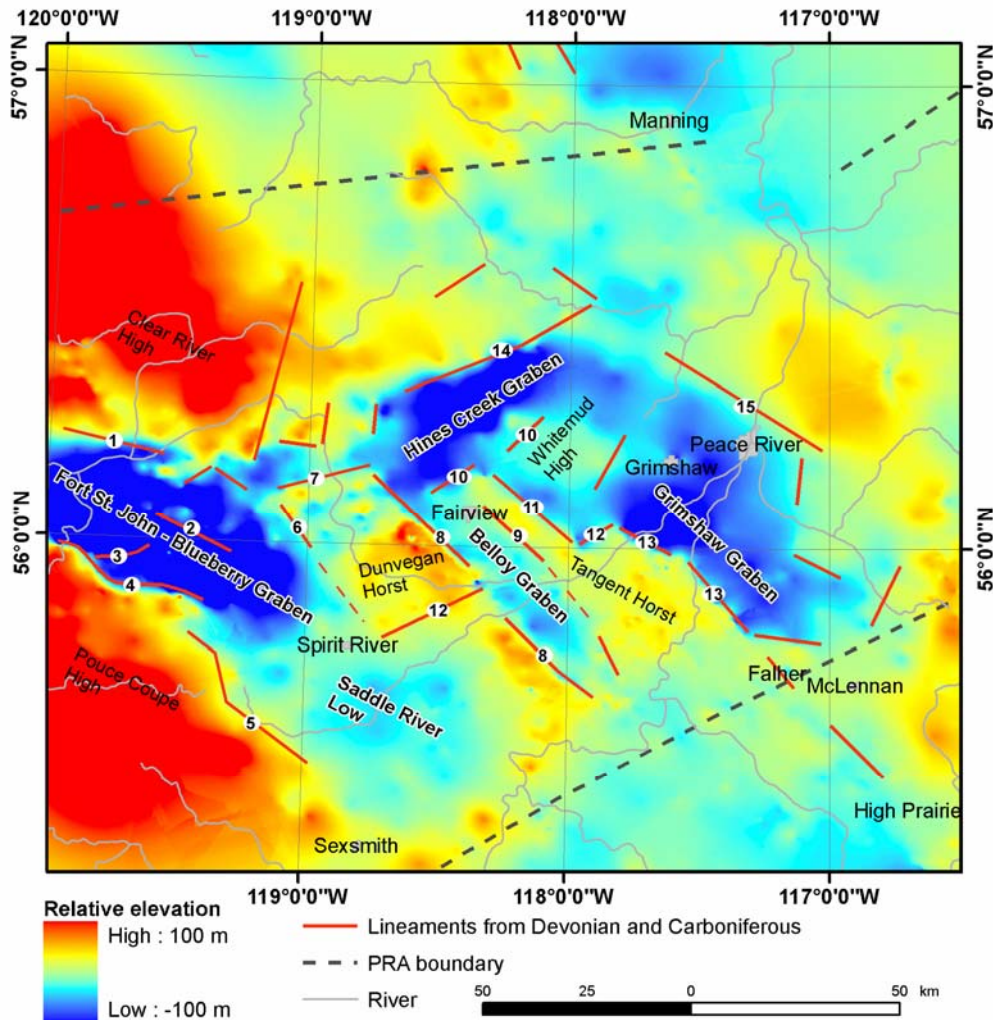
Figure 1. Refined interpretation of the Dawson Creek graben complex (DCGC), superimposed on the residual map for the top of the Debolt Formation. Major faults: 1, Bear Canyon; 2, Josephine Creek; 3, Farmington; 4, Gordondale; 5, Saddle Hills; 6, Rycroft; 7, George; 8, Belloy (Dunvegan); 9, Fairview; 10, Whitemud; 11, Bluesky; 12, Berwyn; 13, Normandville (Tangent); 14, Hines Creek; 15, Peace River.
