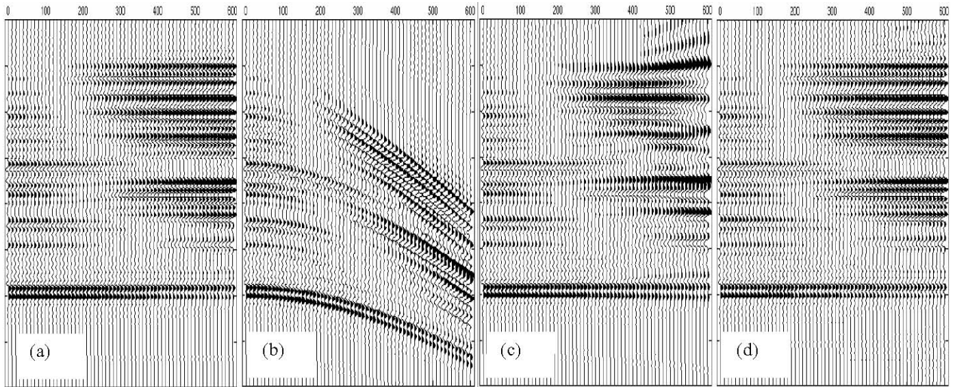
Figure 1. NMO stretching and tuning correction for an offset gather with strong AVO effect. (a) ideal gather, no stretching, no normal moveout applied. (b) before NMO correction; (c) after NMO correction. Stretching can be seen. (d) after stretching and tuning corrections applied on (c). AVO is restored at far offset traces after stretching and tuning corrections.
