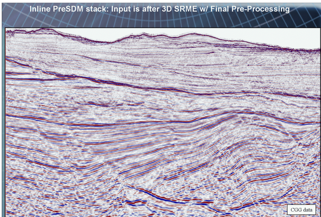
Figure 4. PreSDM using final demultiplied gathers as input
