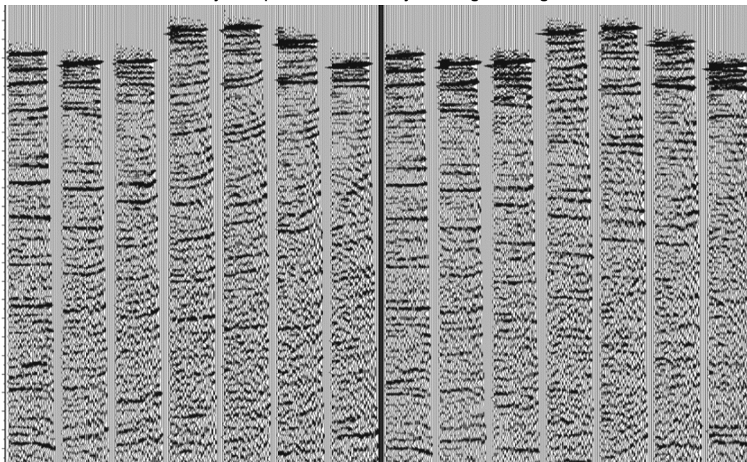
Figure 2. PreSDM Gathers after Iteration-1 (LHS) vs after iteration-2 (RHS) -Note how quickly the velocities (and the residual moveout) vary across the line.
