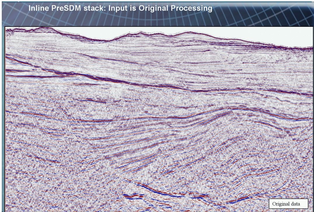
Figure 3. PreSDM using original gathers as input
