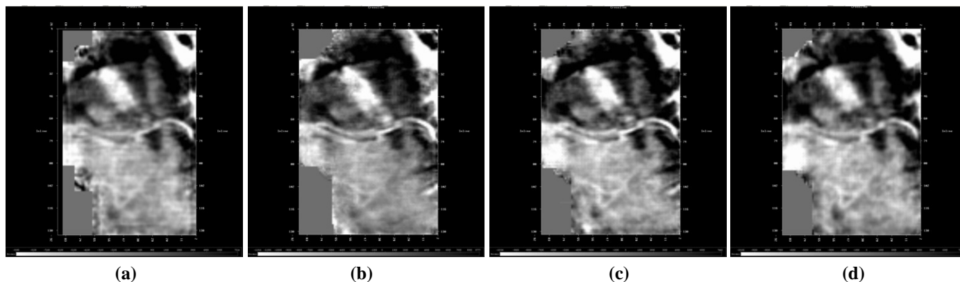
Figure 4: Time slices. a) Post-stack migration on decimated data after post-stack interpolation, b) PreSTM of original data, c) COV PreSTM on original data, d) COV PreSTM of 5D interpolated data.
