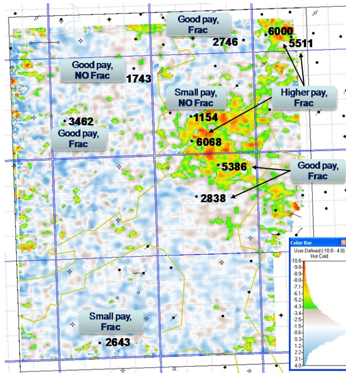
Figure 3: Anisotropy from time difference between P-S1 and P-S2 interpreted top Gravelbourg horizon (warm colours corresponding to larger time differences). Comparable wells with three month total fluid production figures are also shown. Note that there is a good correlation between areas of high shear-wave anisotropy and wells which responded well to fracturing.
