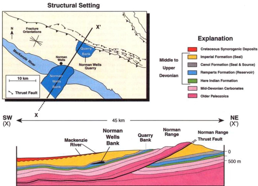
Figure 2: Structural framework of Norman Wells, reproduced from Yose et al. (2001).
