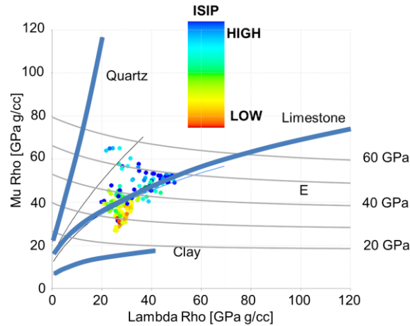
Figure 7. LMR crossplot of seismically derived seismic rock properties color coded by ISIP.
