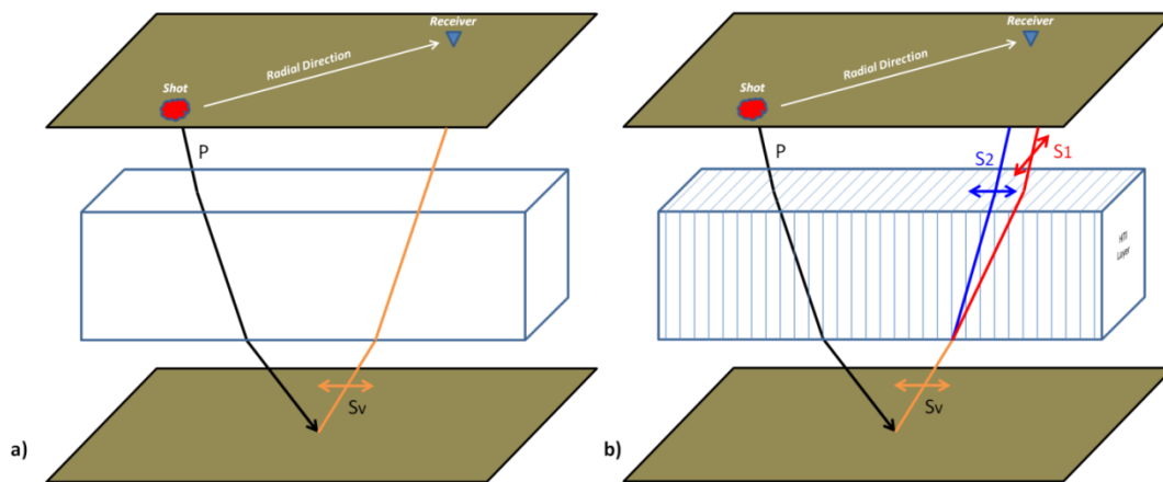
Figure 2 Shows the concept of converted wave splitting in HTI media. Without HTI anisotropy the wave propagates without splitting (a). With HTI anisotropy the converted wave splits into two modes, labelled S1 and S2 (b). The layering can be thought of as vertical fracturing or regional direction of maximum horizontal stress in the absence of fractures. (Wikel et al, 2012)
