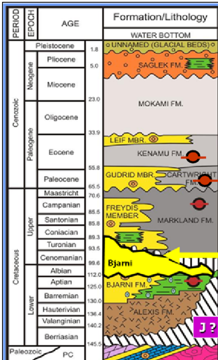
Figure 5: Canadian Labrador basins Stratigraphic column (after Enachescu, 2011).
