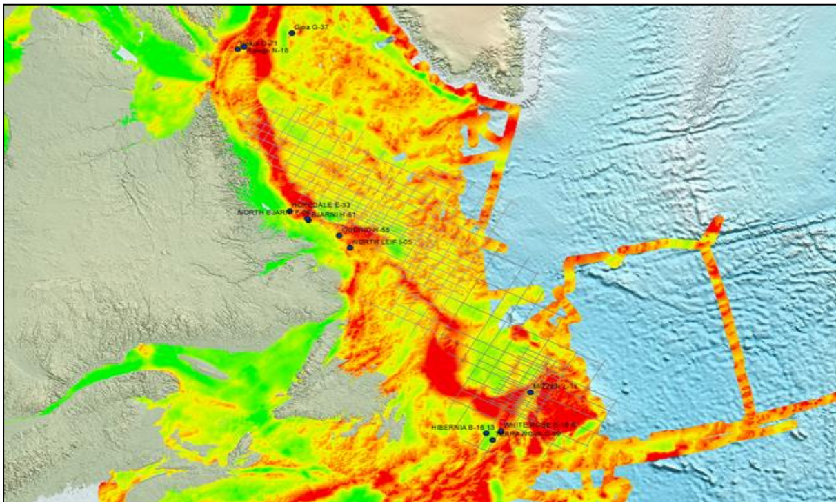
Figure 3: Key wells, GeoStreamer survey and free air gravity (Green denotes gravity low which equates to thicker sediments)
