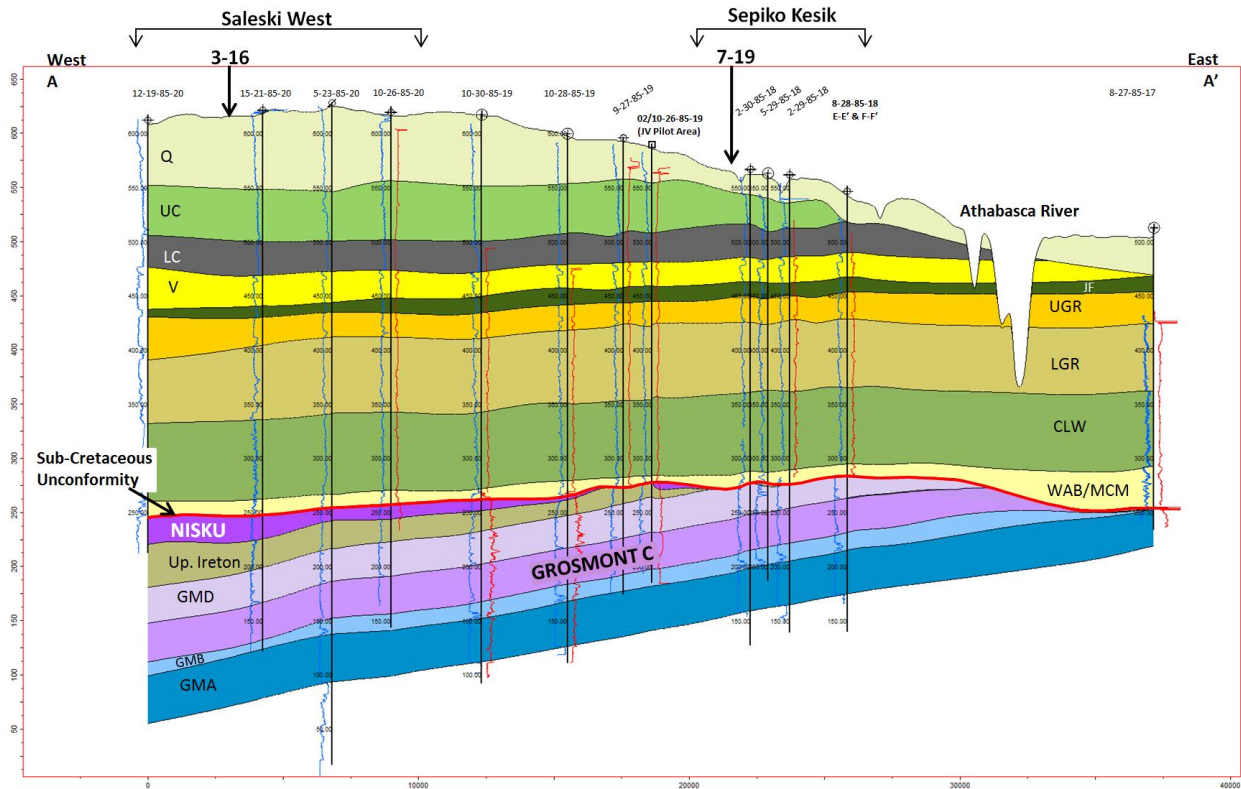
Figure 2. Cross-section across study area.
