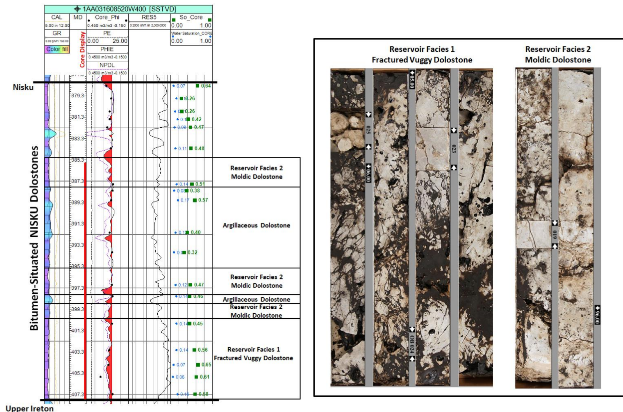
Figure 4. Nisku Formation reference well 3-16.
