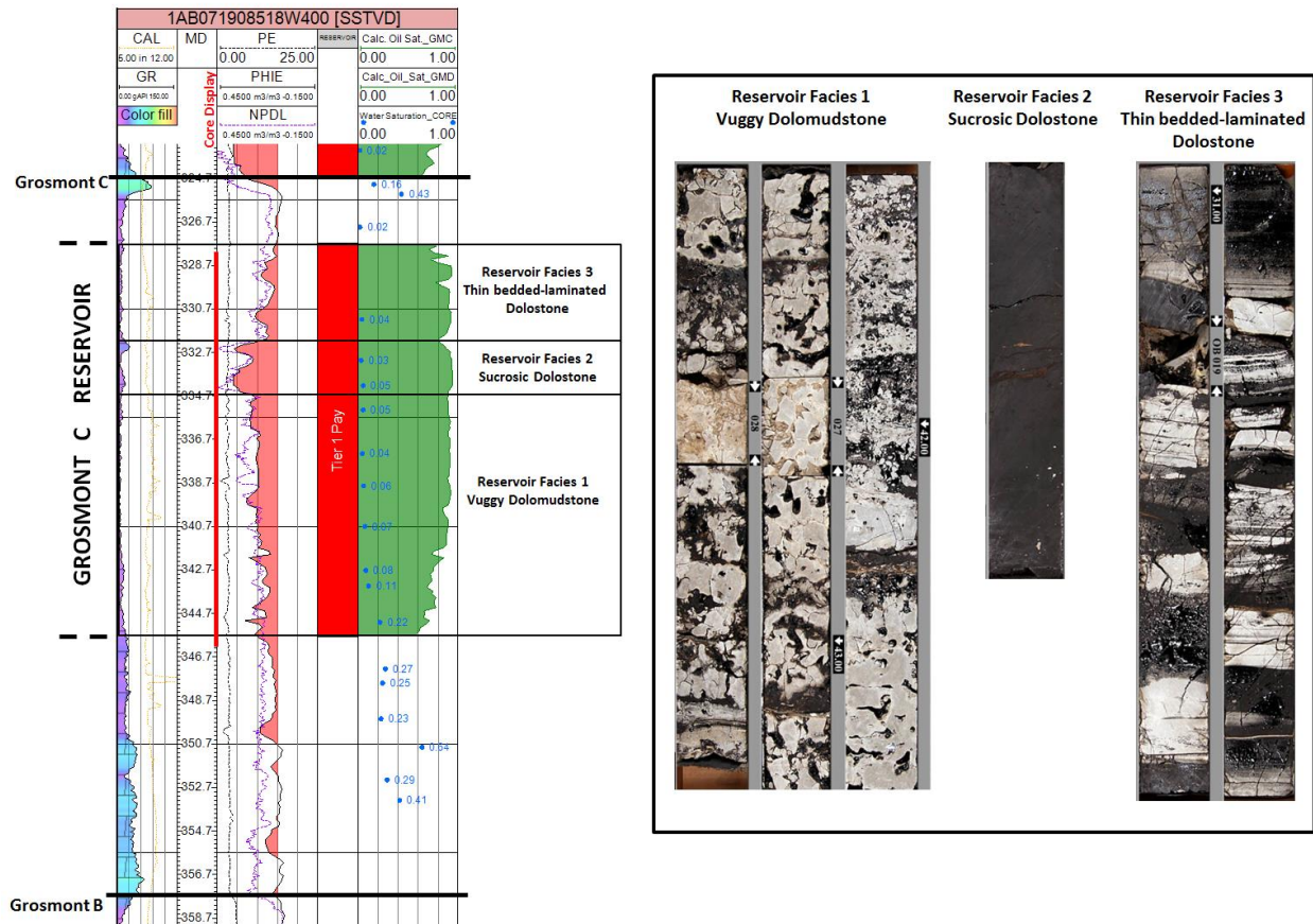
Figure 3. Grosmont C reference well 7-19.
