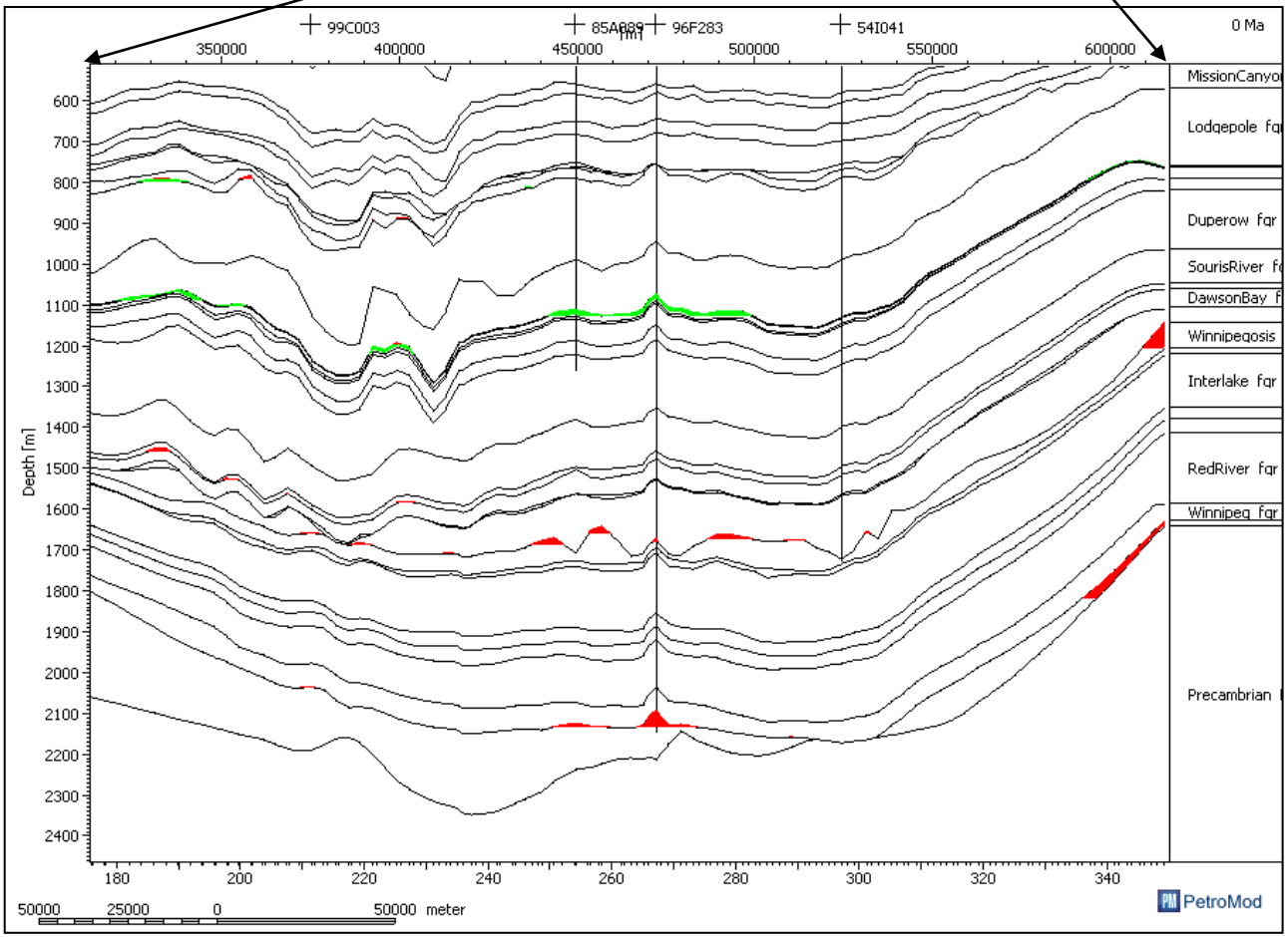
Figure 9. 2D model along transect A - A' showing oil (green) and condensate/light oil/liquid vapor migration (red) accumulation in mostly structural traps. The model replicates existing pools
