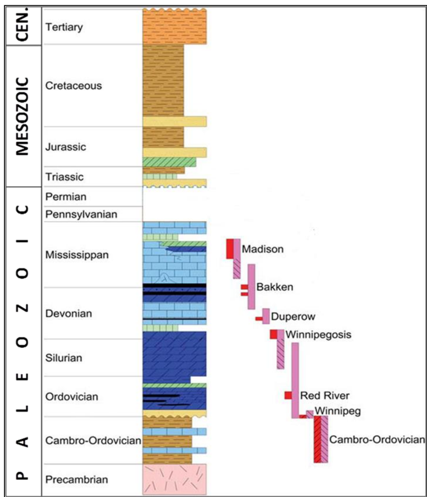
Figure 2. Generalised stratigraphic column showing the stratigraphic range of the Paleozoic petroleum systems in the Northern Williston Basin subsurface. Source rock range (red), reservoir rock range (pink), while hashed intervals represent questionable or speculative ranges (modified from Nordeng, 2013)
