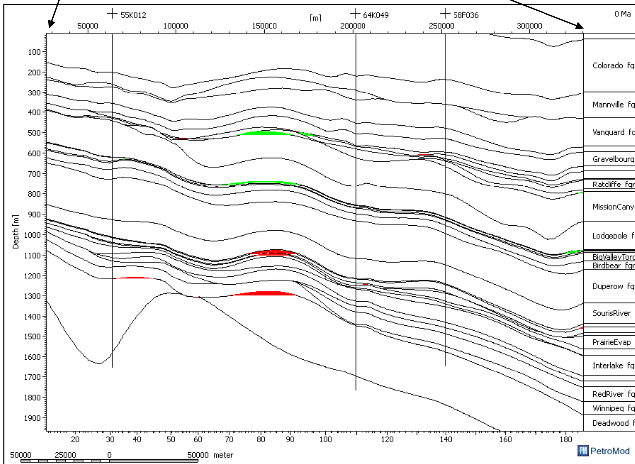
Figure 10. 2D model along transect A - A' showing oil (green) and condensate/light oil/liquid vapor migration (red) accumulation in mostly structural traps. The model shows potential hydrocarbon pools
